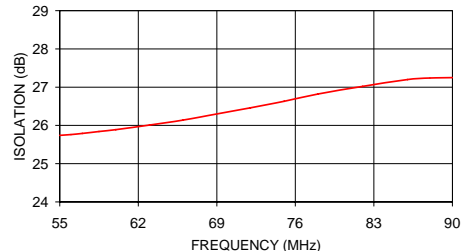
SCPQ-90 ISOLATION
